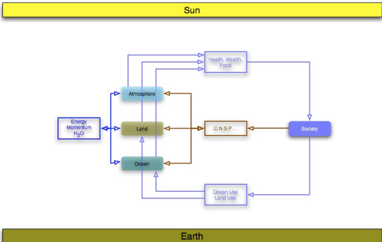
Figure 1: Schematic view of the major components of the Earth system: atmosphere, land and ocean, society and a number of coupling agents between the components. The physical climate system is driven by fluxes of momentum, energy and includes the hydrological cycle. Substances like carbon C, nitrogen N, sulfur S, phosphor P are important for the regulation of the fluxes of energy, momentum and water, for example by their role in the atmospheric radiative balance (by CO 2 ), or as a key substance in biology (P). Amounts and distribution of such key substances can be modified by humanity as a by-product of economic activity, which may also alter the environment by the use of land and ocean resources. Society itself is striving for life quality - for values like health, wealth or simply enough food and water, which depend on the climate and its variability or trends. Earth system models aim at the representation of the physical, chemical and biogeochemical system and its interaction with society as outlined here.
