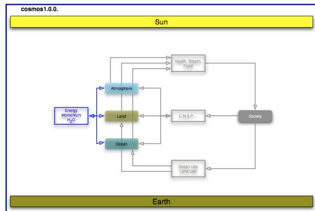
Figure 2: COSMOSv1.0.0 represents the physical climate system considering atmosphere, land and ocean. These components interact by fluxes of energy, momentum and water, including a closer hydrological cycle. Society and material fluxes are planned to be included in later versions. See also Fig. 1.
